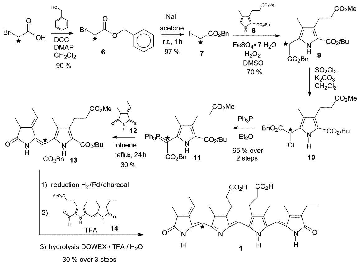
Scheme 2. Synthesis of 5- ^{13}\text{C} PCB. Bn: benzyl.
