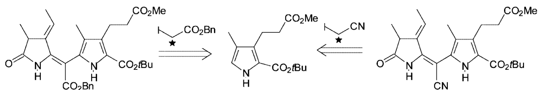
Figure 2. Retrosynthetic proposal for introduction of ^{13}\text{C} -label into position 5 of PCB ( 1 ).
