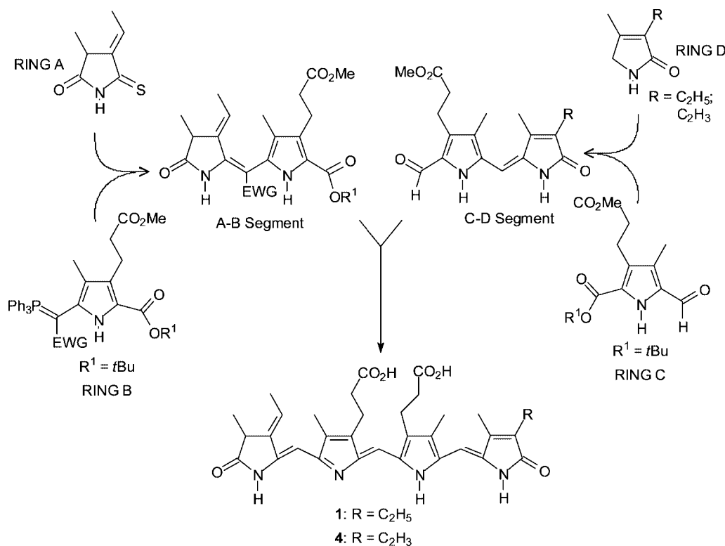
Scheme 1. Overview of the chemical synthesis of compounds 1–5 . EWG: electron-withdrawing group.
