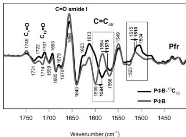
Figure 3. FTIR difference spectrum ( P_{fr} - P_r ) of 10\text{-}^{13}\text{C} -labelled \text{P}\Phi\text{B} , incorporated into apo phyA of oat (65 kDa N-terminal domain). Positive bands are assigned to the photoproduct ( P_{fr} ) whereas negative bands are related to the P_r form. Changes due to the isotope shift are indicated by arrows.
