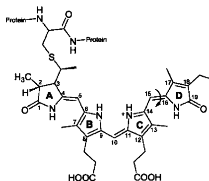
Figure 1. Structural formula of phycocyanobilin (1), covalently bound to cysteine321 of oat phytochrome. Attachment is accomplished through position 3' in the A-ring, which in unbound form is part of an ethylidene substituent. The chromophore is shown in ZZZ,asa form. Phytochromobilin differs from PCB only in the substituent at position 18 (vinyl vs. ethyl). The photoisomerization of the 15–16 double bond is indicated by an arrow.
